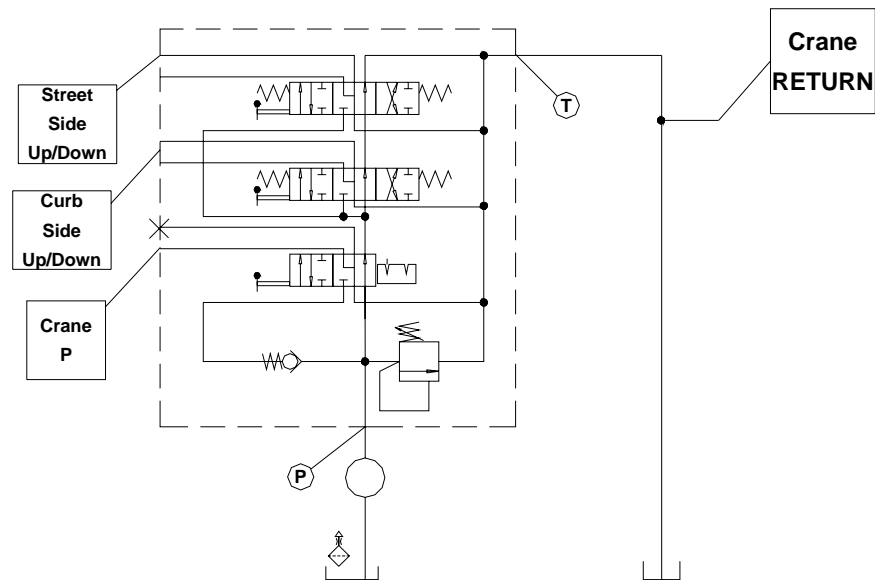
HYDRAULIC SCHEMATIC
